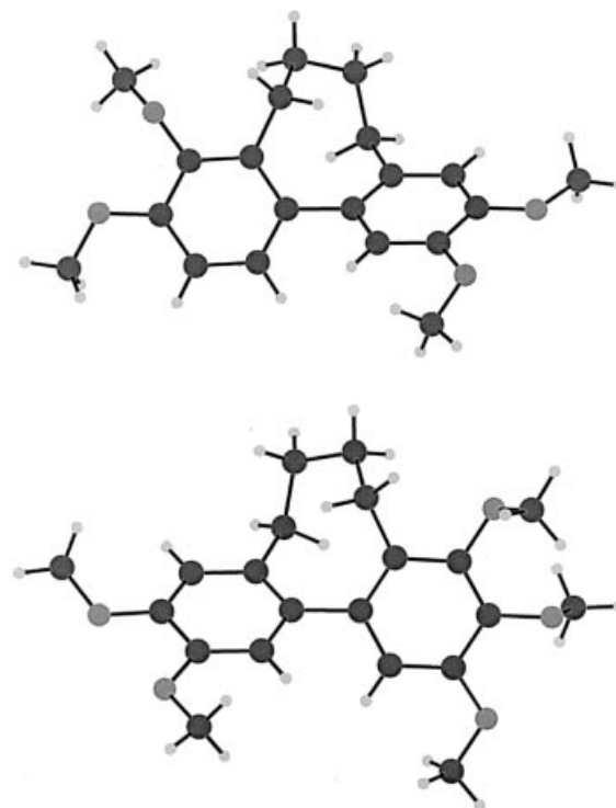
Figure 2. Structures of 5f (top) and 5g (bottom) in the crystal
