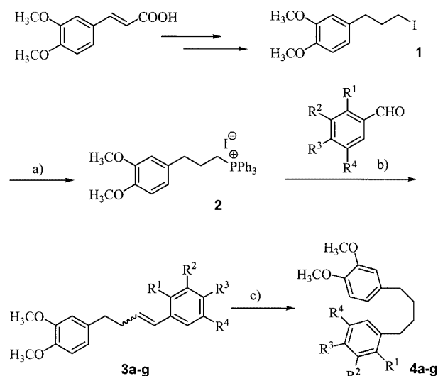
Scheme 1. a) \text{PPh}_3 , DMF, reflux; b) i. \text{KOtBu} , THF, 0^\circ\text{C} , ii. benzaldehyde derivative; c) \text{Pd/C} , \text{H}_2 , THF, room temp.
