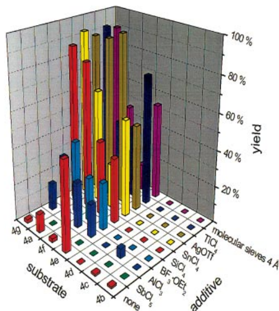
Figure 1. Screening for additives in the MoCl 5 -mediated oxidative coupling reaction
