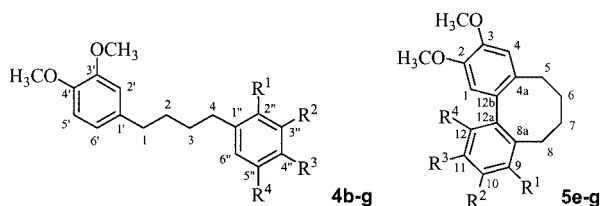
Scheme 3. Systematic numbering of the carbon atoms in the 1,4-diarylbutanes and 2,2'-cycloolignans
