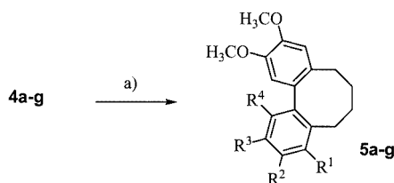
Scheme 2. a) \text{MoCl}_5 , additive, \text{CH}_2\text{Cl}_2 , 0^\circ\text{C}
